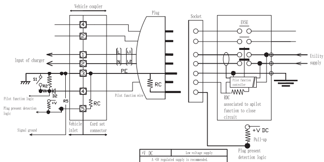
Figure 1: Example for the simultaneous proximity detection and current coding function
