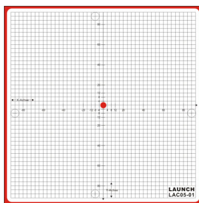
Fig. 5-9 (Magnetic laser)
