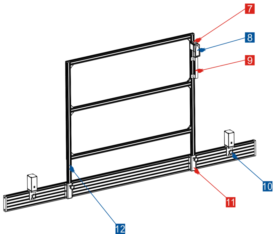
Fig. 3-4b Rear view
