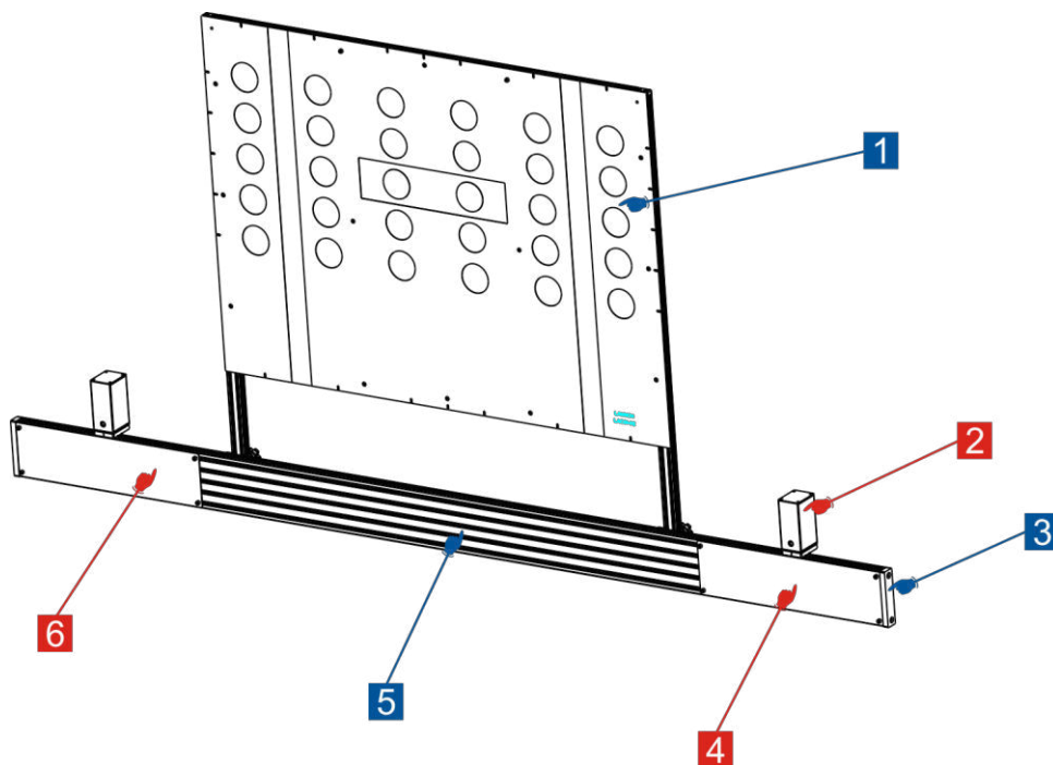
Fig. 3-4a Front view
